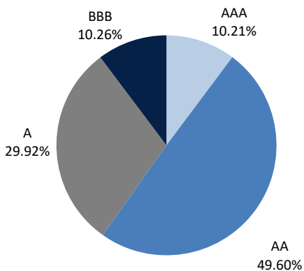
CREDIT PROFILE 5
