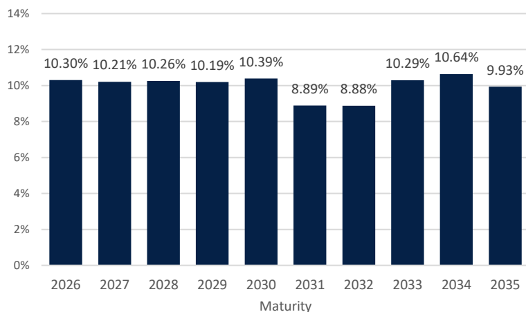
MATURITY PROFILE
